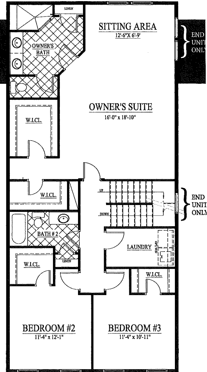
SECOND FLOOR WITH THIRD FLOOR OPTION
