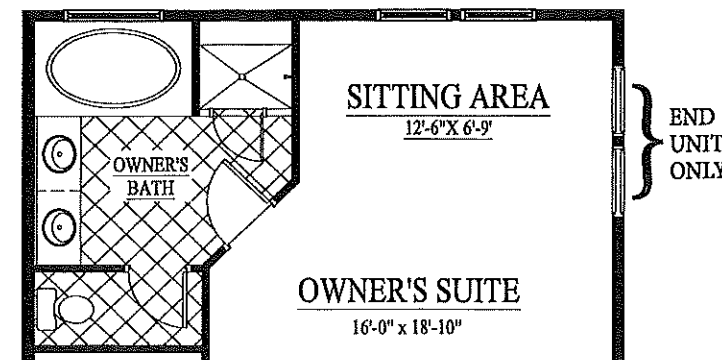
OPTIONAL OWNER'S BATH
